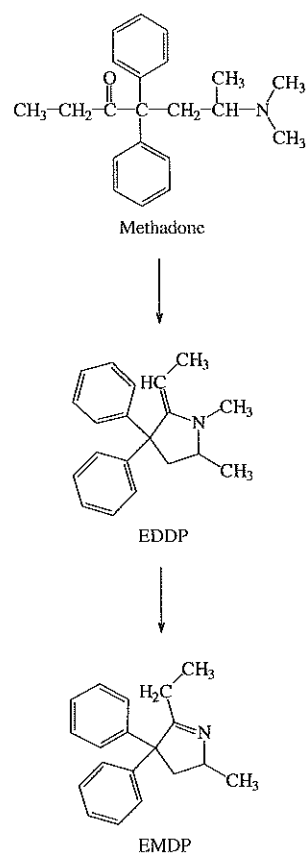
Figure 31-29 Metabolism of methadone.
