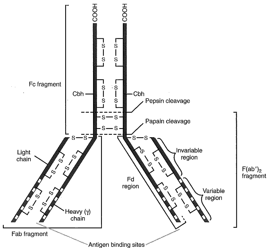
Figure 10-1 Schematic diagram of IgG (immunoglobulin G) antibody molecule showing carbohydrate (Cbh), disulfide bonds (SS), and major fragments produced by proteolytic enzyme treatment ( F(ab')_2 , Fc, Fab, Fd).
