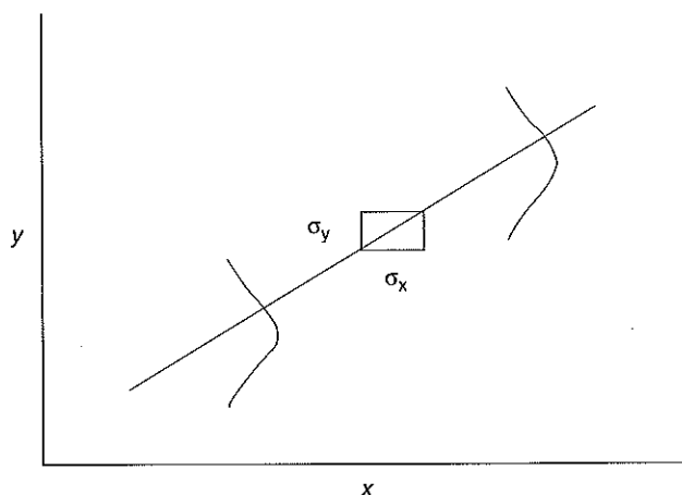
Figure 13-6 Relation between concentration ( x ) and signal response ( y ) for a linear calibration curve. The dispersion in signal response ( \sigma_y ) is projected onto the x axis giving rise to assay imprecision ( \sigma_x ).
