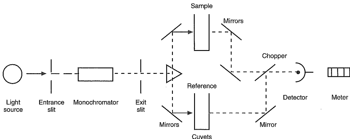
Figure 4-5 Double-beam-in-time spectrophotometer.
