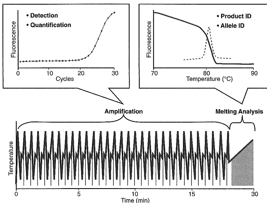
Figure 17-17 Real-time monitoring during amplification and melting analysis.
