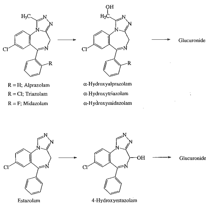
Figure 31-17 Metabolic transformation of some triazolobenzodiazepines.
