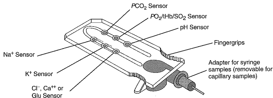
Figure 12-5 Schematic view of the measurement cassette for the OPTI Medical Critical Care Analyzer. (Courtesy OPTI Medical, Roswell, GA.)
