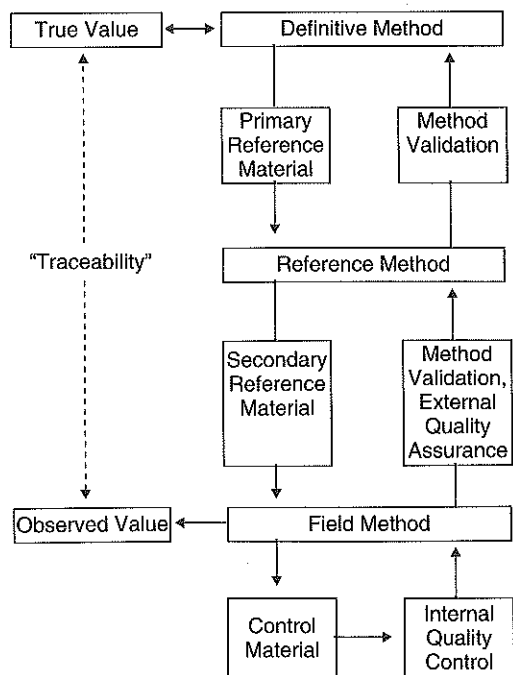
Figure 16-9 Structure of an accuracy-based measurement system showing relationships among reference methods and materials.
