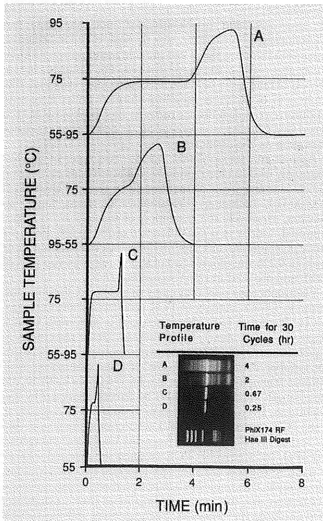
Figure 17-11 Rapid PCR improves product specificity. Samples were cycled 30 times through profiles A, B, C, and D. Increased specificity of amplification of a 534 bp \beta -globin fragment is seen with faster cycles (C and D). (Reprinted with permission of Eaton Associates.)
