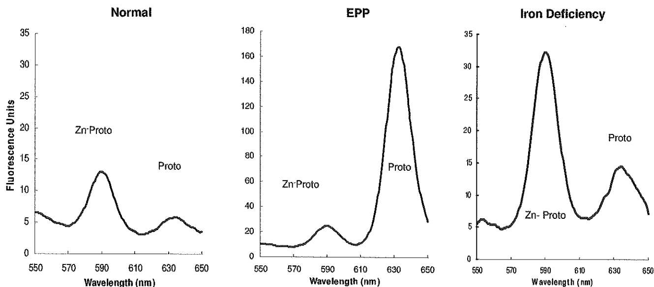
Figure 29-3 Fluorescence emission spectra (excitation at 405 nm) of ethanolic extracts of erythrocytes from a normal individual and patients with lead toxicity and erythropoietic protoporphyria (EPP). Note that different scales are used.
